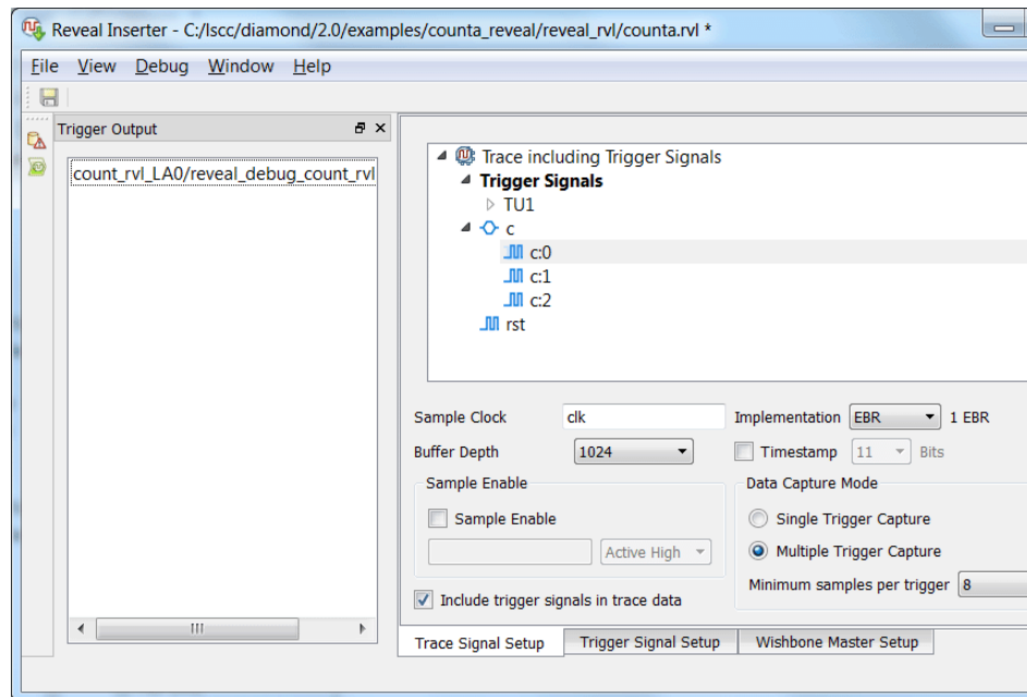
Figure 98: Reveal Inserter Trace Signal Setup
