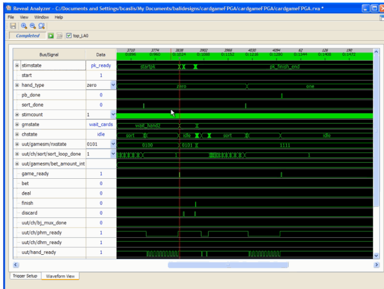
Figure 103: Reveal Analyzer Waveform View
