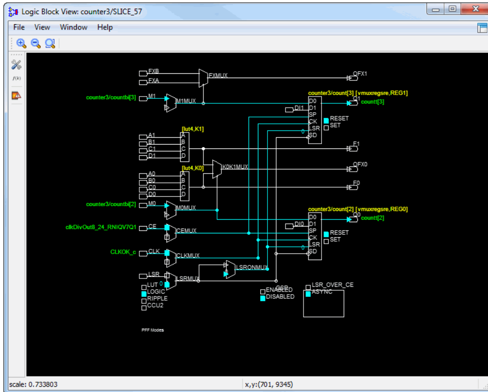
Figure 107: Logic Block Schematic View
