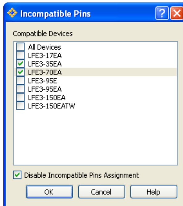
Figure 129: Incompatible Pins Dialog Box
