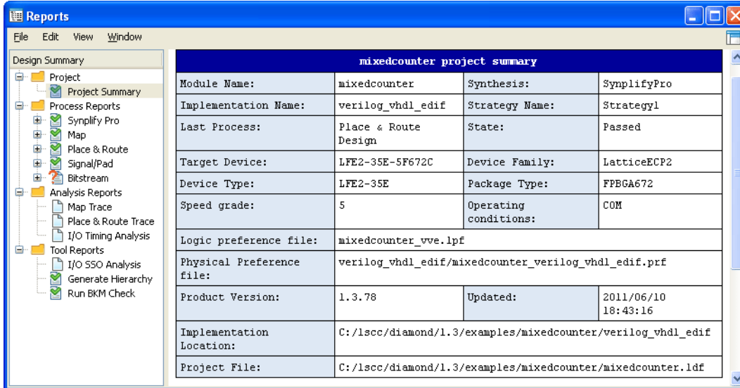
Figure 83: Reports View
