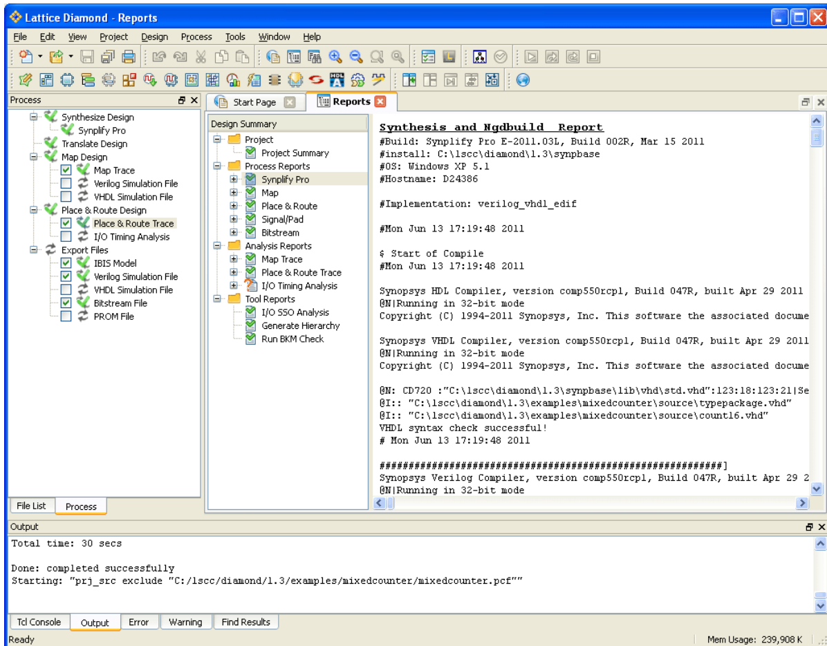
Figure 116: Synthesis Report
