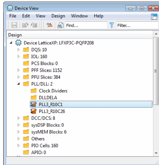
Figure 89: Device View
