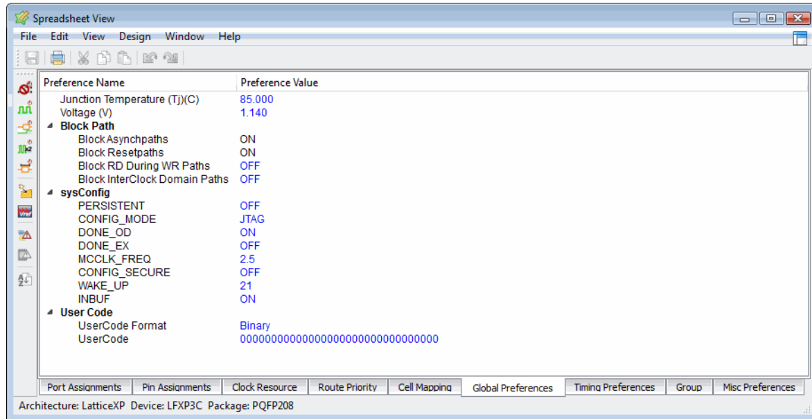
Figure 85: Spreadsheet View
