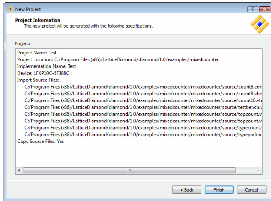
Figure 9: Project Summary
