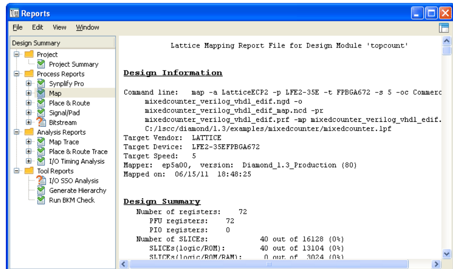
Figure 42: Reports View
