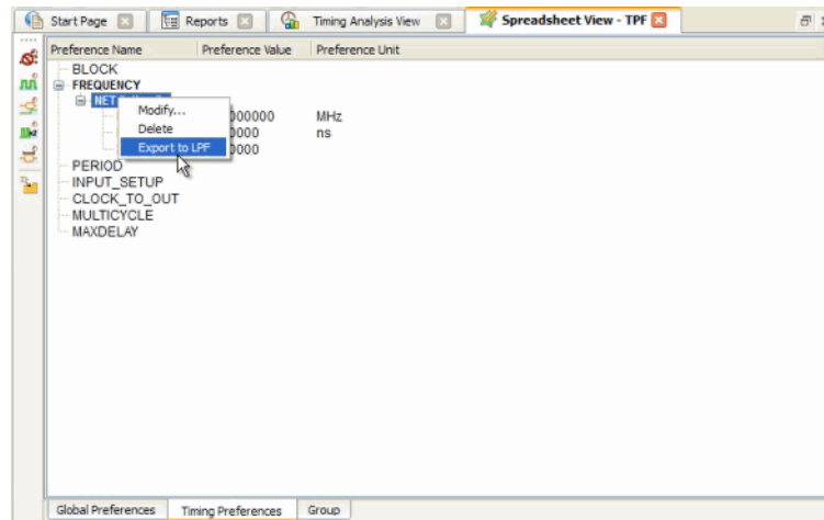
Figure 110: Export TPF
