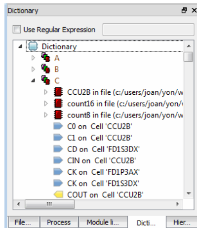
Figure 39: Dictionary View
