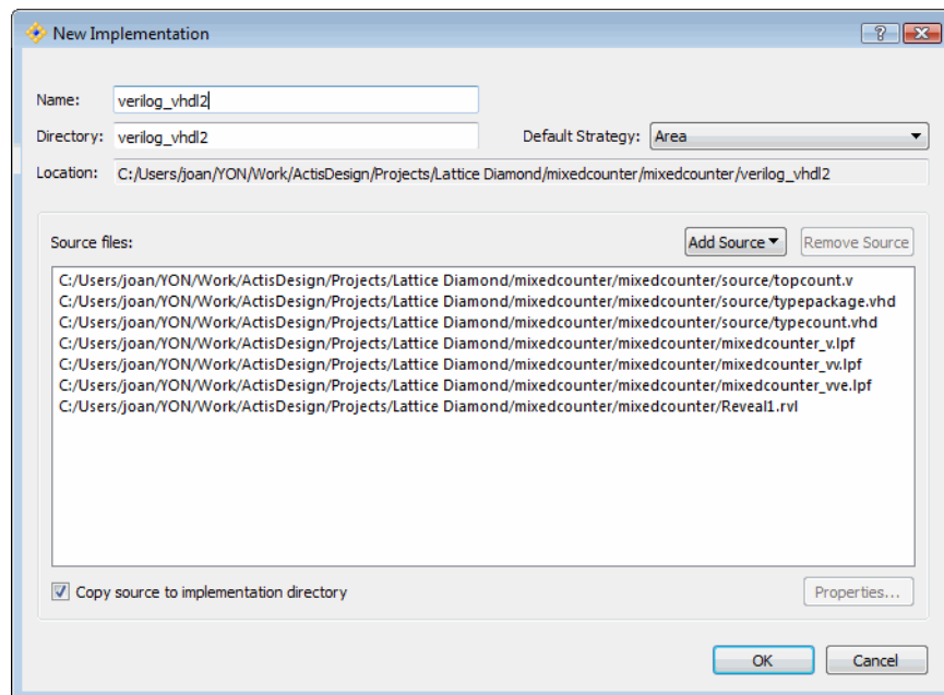
Figure 60: New Implementation
