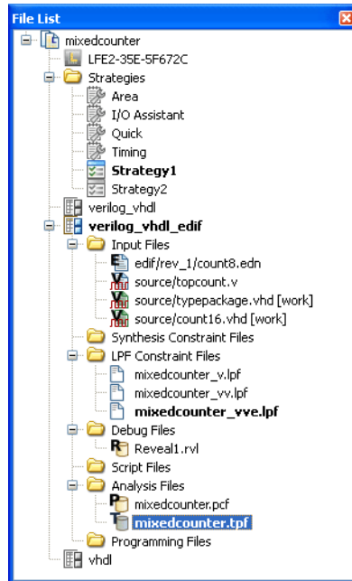
Figure 107: Timing Analysis Preference File
