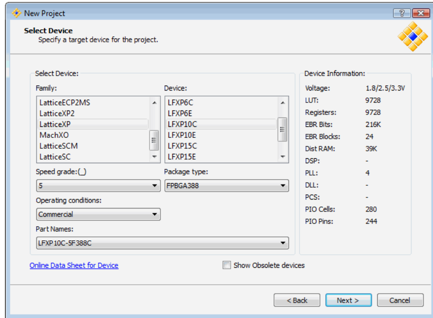
Figure 8: Select Device
