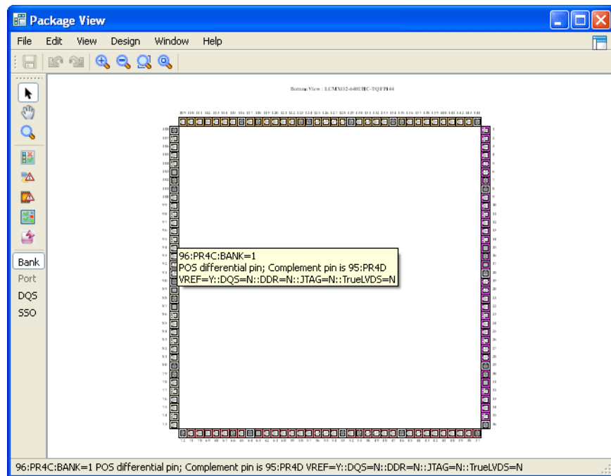
Figure 88: Package View
