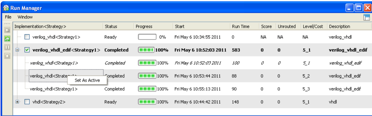
Figure 115: Run Manager
