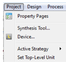
Figure 59: Project Menu
