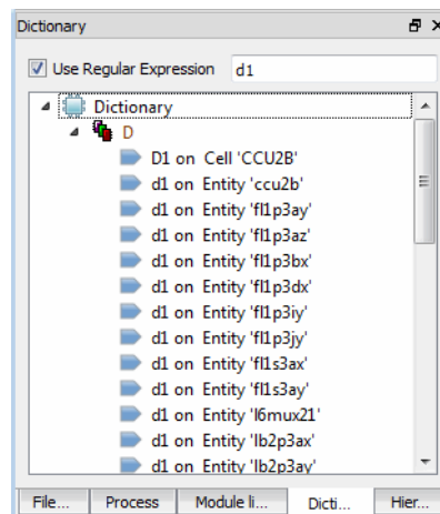
Figure 40: Dictionary View with Regular Expression Filter
