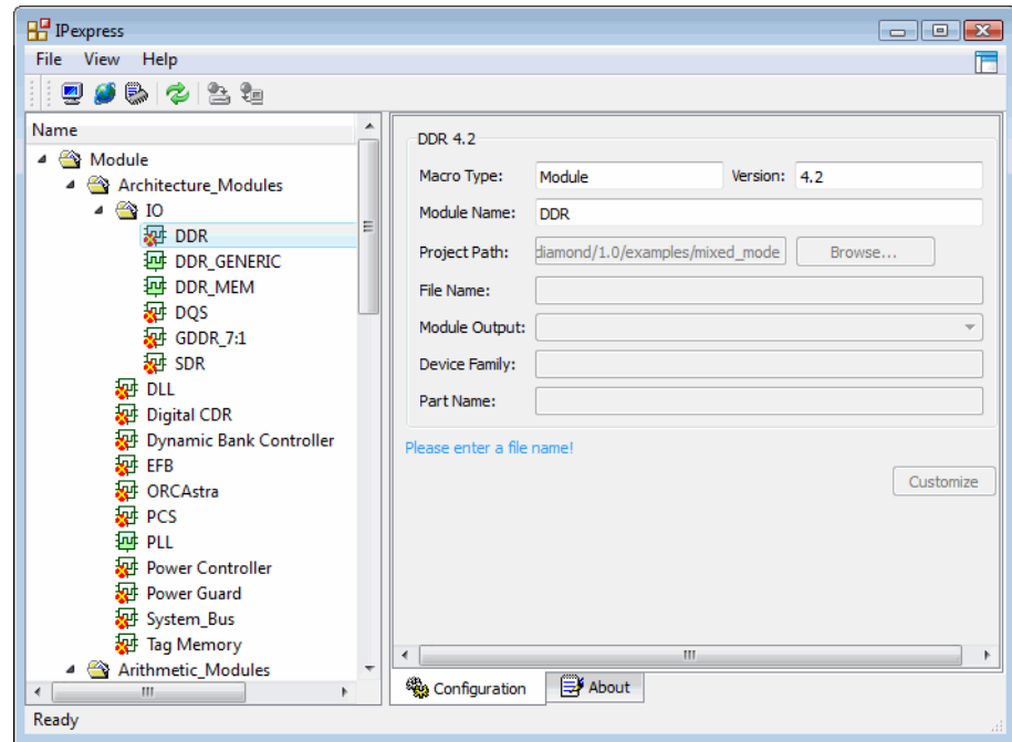
Figure 95: IPexpress
