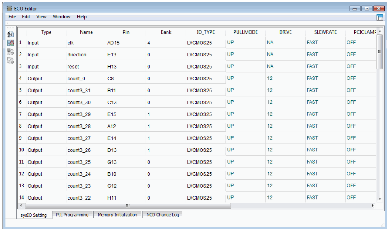
Figure 113: ECO Editor
