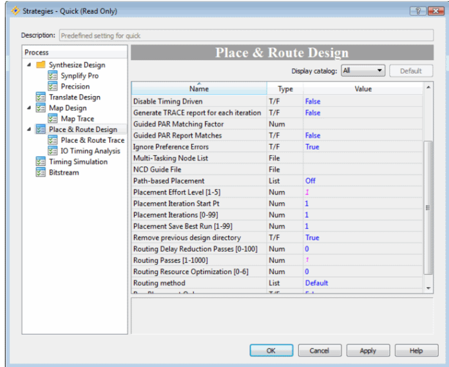
Figure 69: Quick Predefined Strategy
