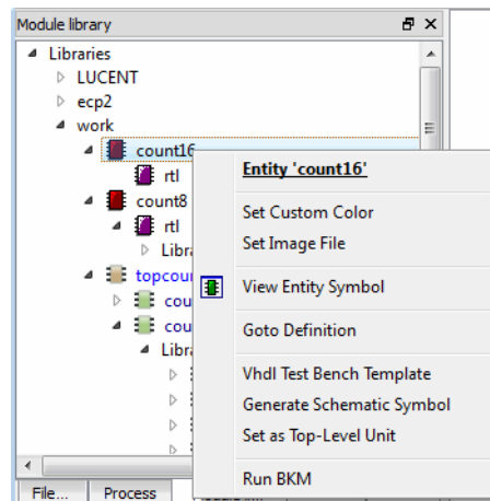
Figure 38: Module Item Description and Actions
