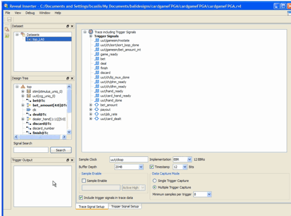
Figure 97: Reveal Inserter Trace Signal Setup
