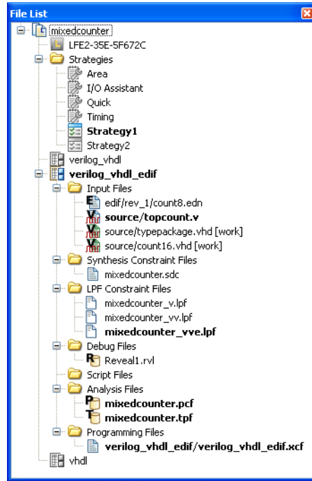
Figure 96: File List View with Reveal Debug Project File
