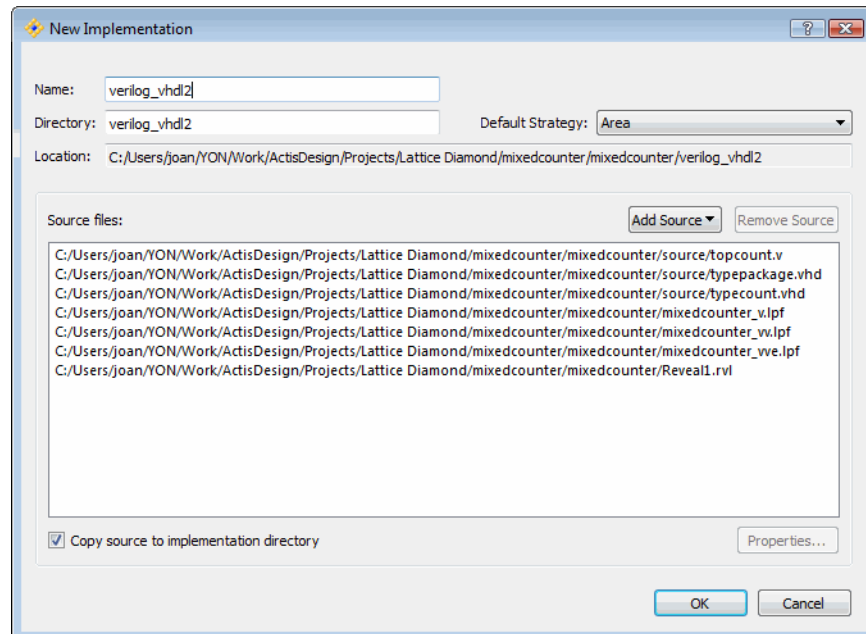
Figure 74: Adding a Source to a New Implementation
