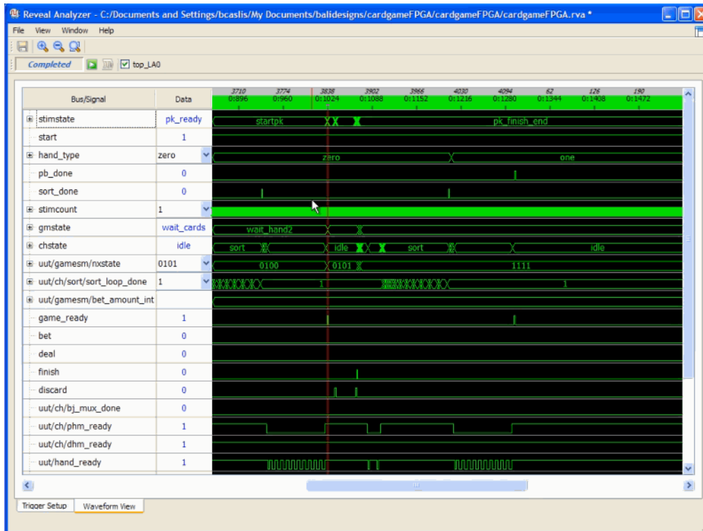
Figure 102: Reveal Analyzer Waveform View
