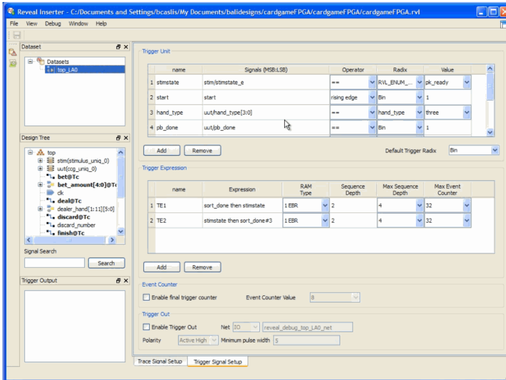
Figure 98: Reveal Inserter Trigger Signal Setup
