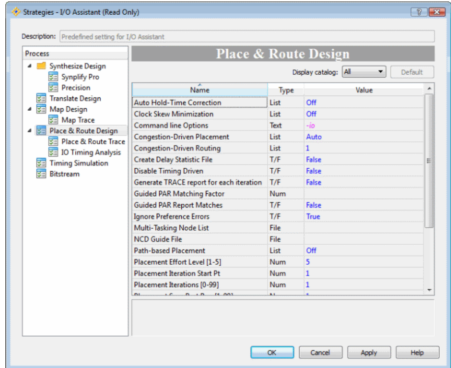
Figure 68: I/O Assistant Predefined Strategy
