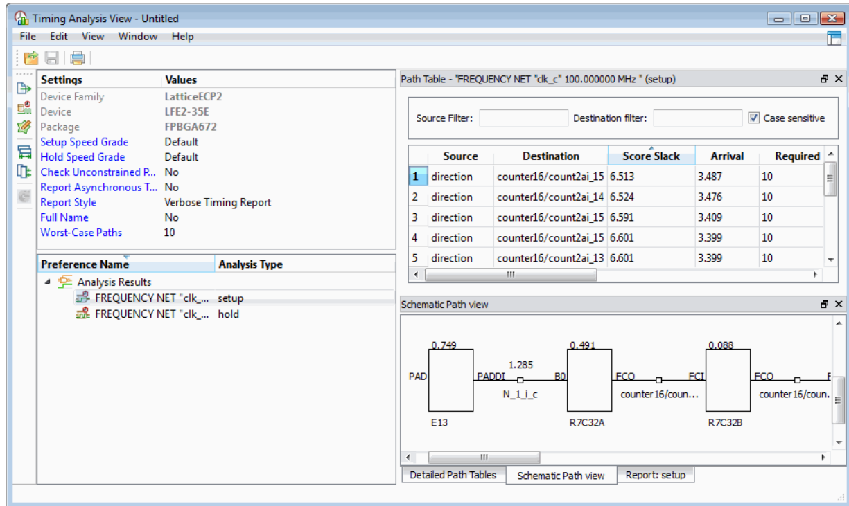
Figure 109: Timing Analysis Schematic Path View
