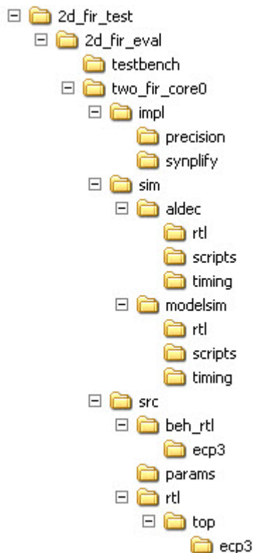
Figure 4-3. 2D FIR Filter IP Core Directory Structure
