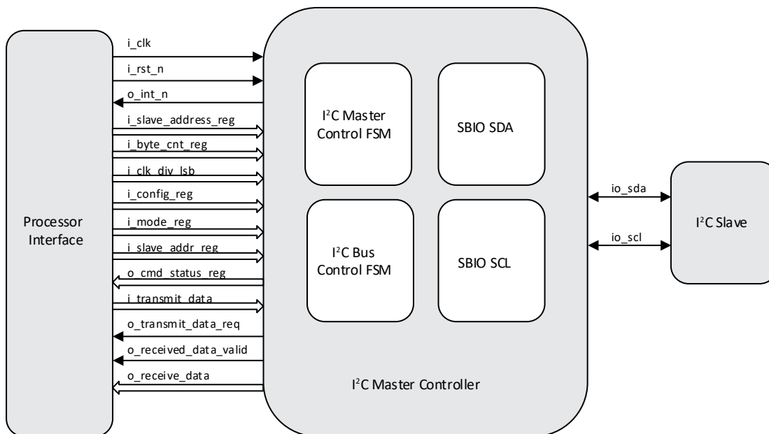
Figure 3.1. Block Diagram
