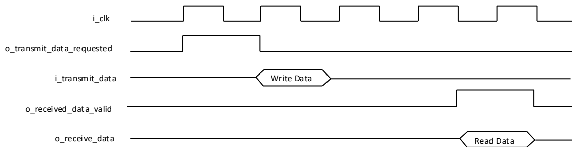
Figure 8.1. Timing Diagram for Read and Write Data Transfer
