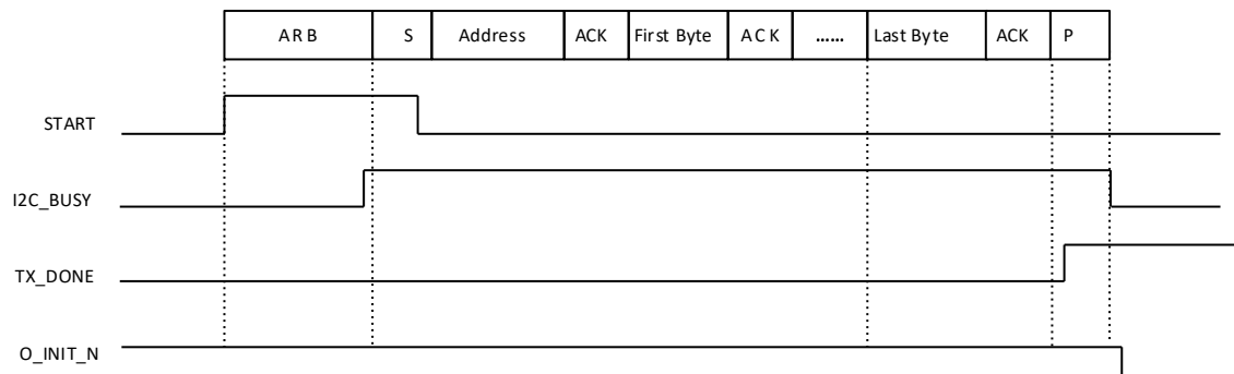
Figure 9.1. Master Transmit Operation
