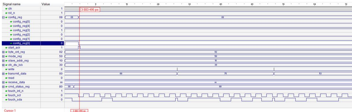
Figure 10.2. Simulation Waveform Showing the START Bit of the Configuration Register and Acknowledge Bit
