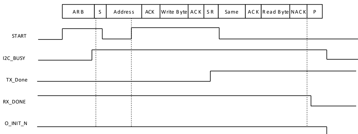
Figure 9.3. Repeated Start Operation
