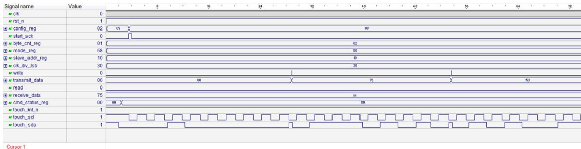
Figure 10.1. HDL Simulation Waveform
