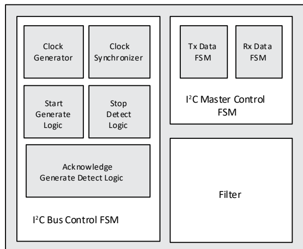
Figure 5.1. Functional Block Diagram
