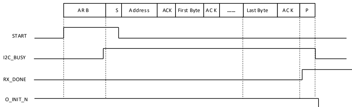
Figure 9.2. Master Receive Operation
