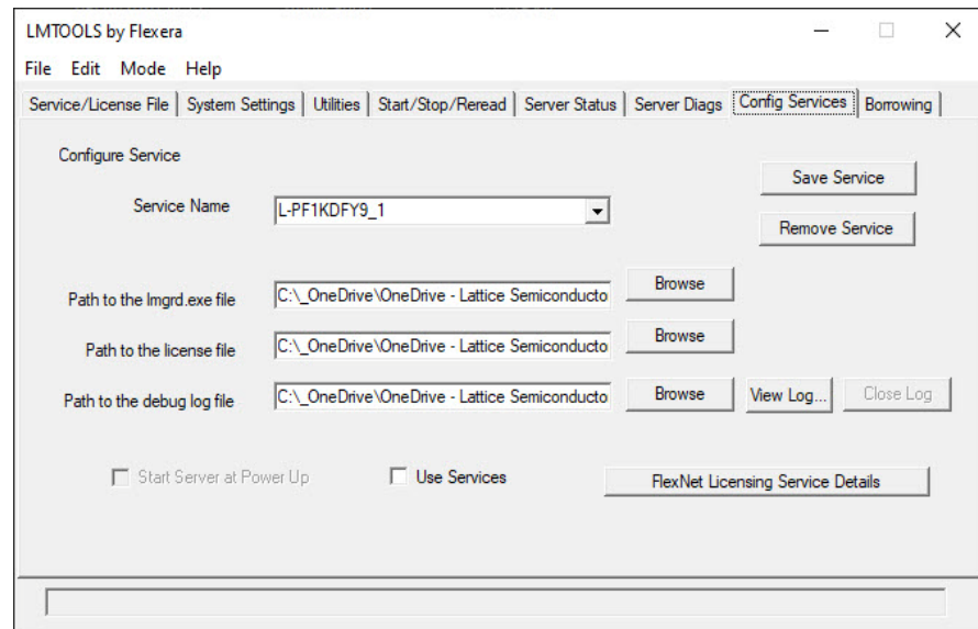
Figure 5: LMTools_Config Services
