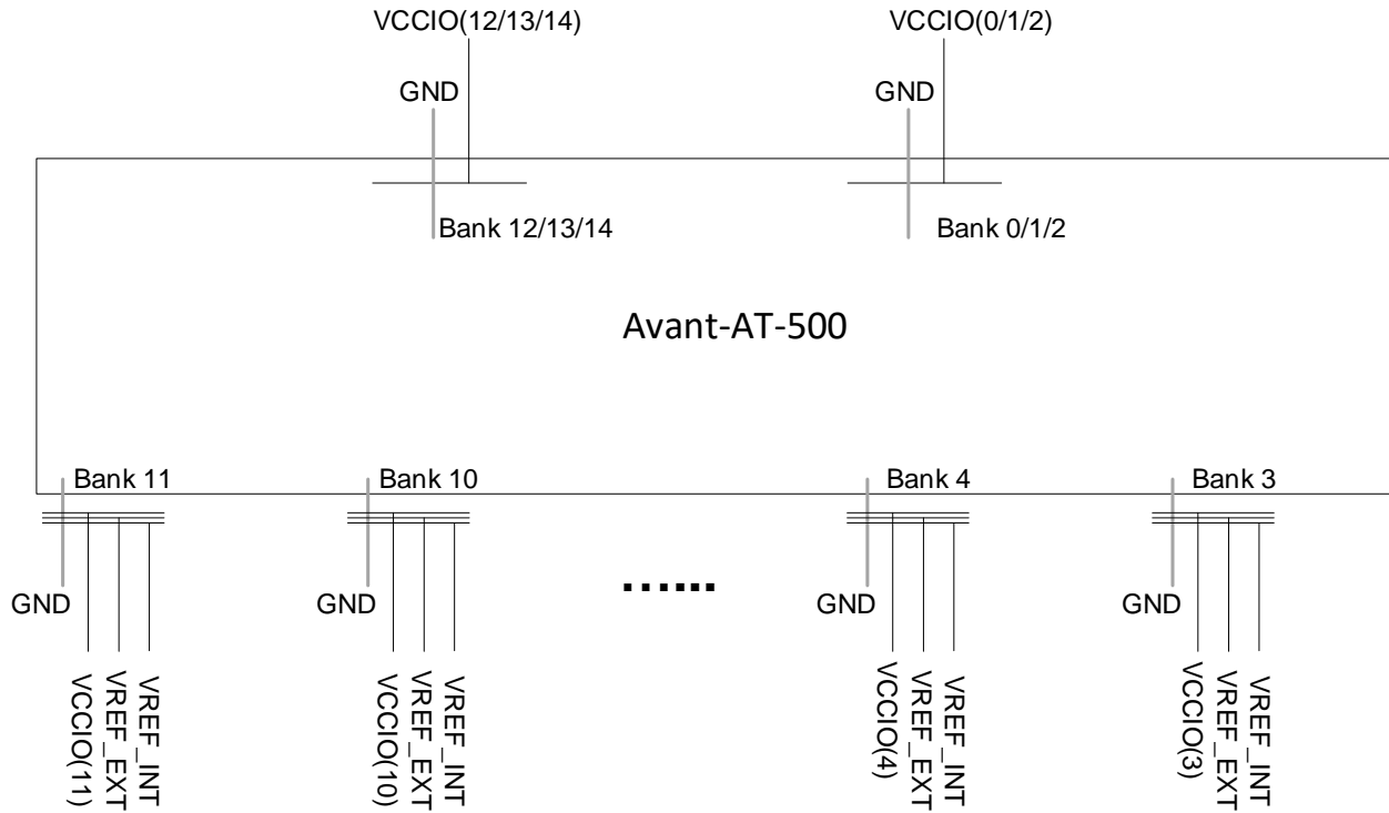
Figure 2.11. sysI/O Banking
