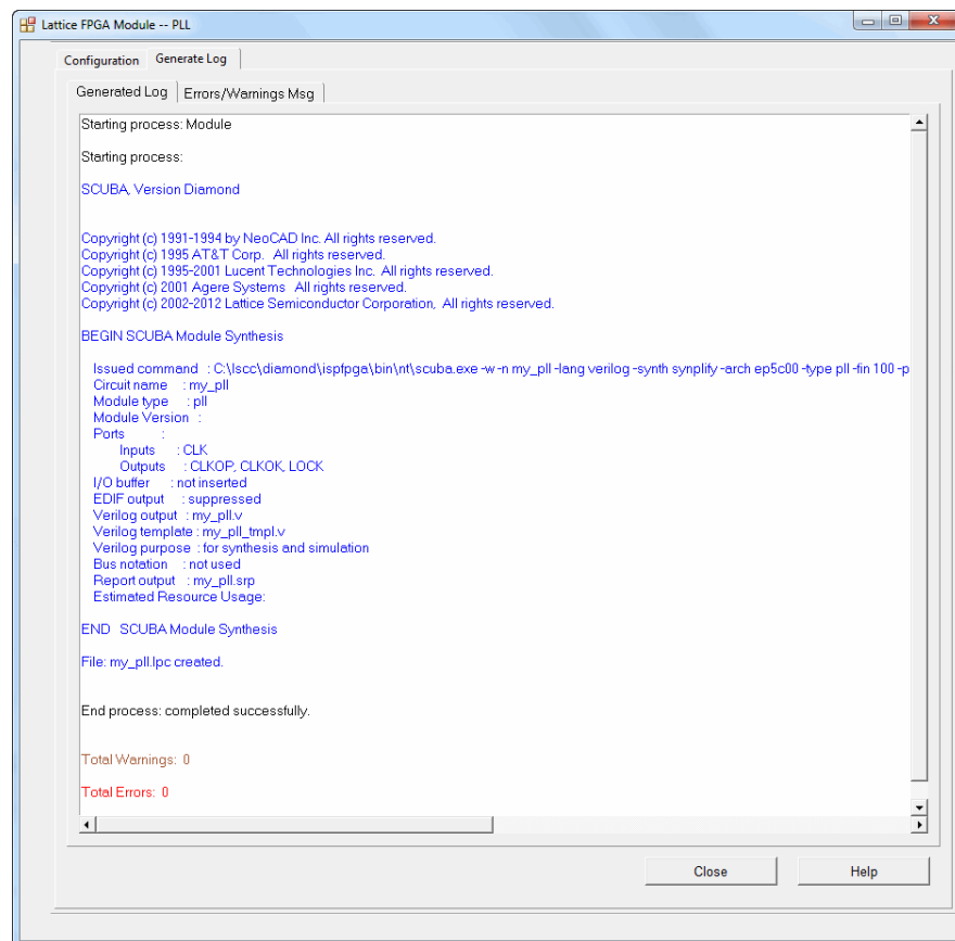
Figure 8: IPexpress Generate Log Tab
