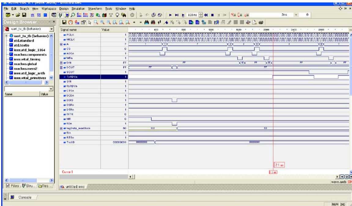
Figure 7 shows the data received on the receiver serial data input line SIN.
