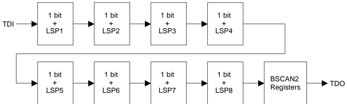
Figure 7. BSCAN2 x 8-Port (Asset Model) LSP Order (All Ports Selected)
