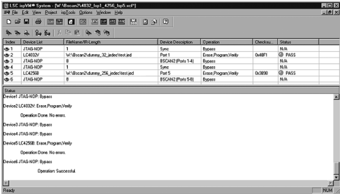
Figure 12. Logical Representation of ispVM Chain Configuration
