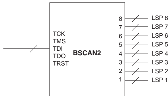
Figure 6. Integrated 8-Port BSCAN2 Implementation
