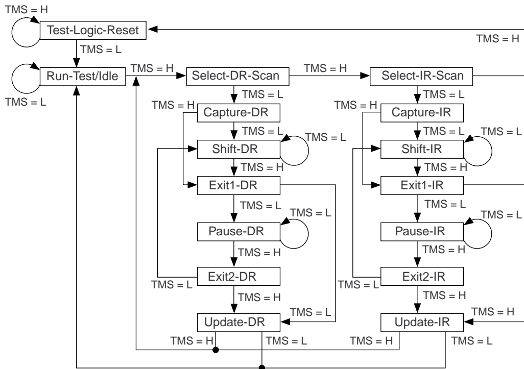
Figure 2. TAP Controller State Machine
