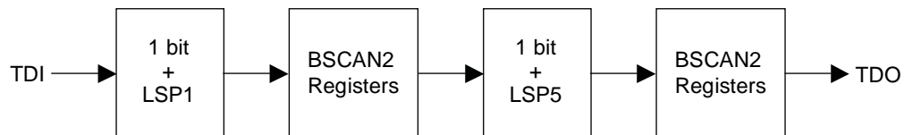
Figure 12. Logical Representation of ispVM Chain Configuration
