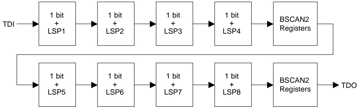
Figure 5. BSCAN2 x 8-Port (JTAG Technologies Model) LSP Order (All Ports Selected)
