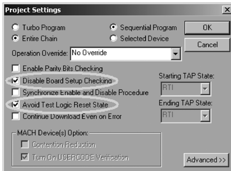
Figure 10. Project Settings for BSCAN2 Compatibility
