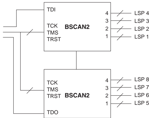
Figure 4. 8-port BSCAN2 Implementation via Daisy Chaining
