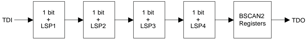
Figure 3. LSP Order (All Ports Selected)
