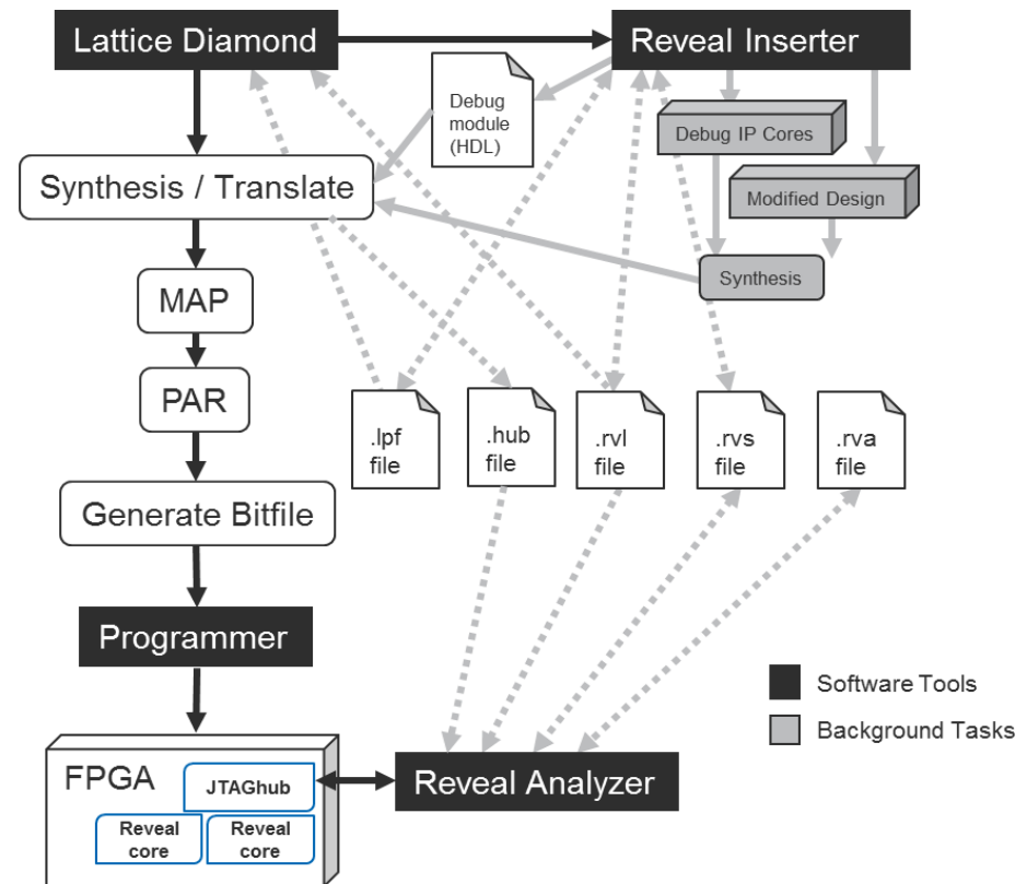
Figure 1: Reveal Inserter Design Flow
