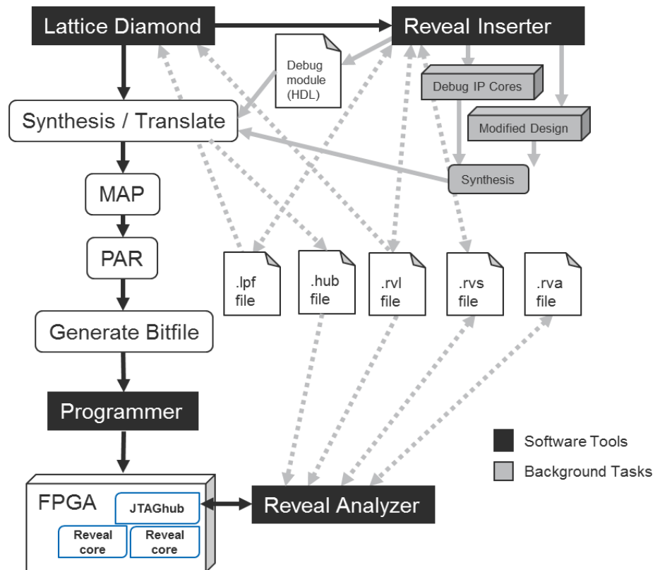
Figure 2: Reveal Design Flow
