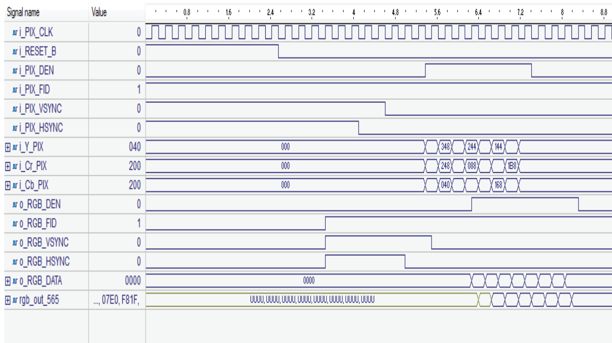
Figure 4. Simulation Waveforms
