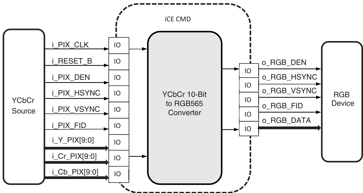
Figure 1. Functional Description
