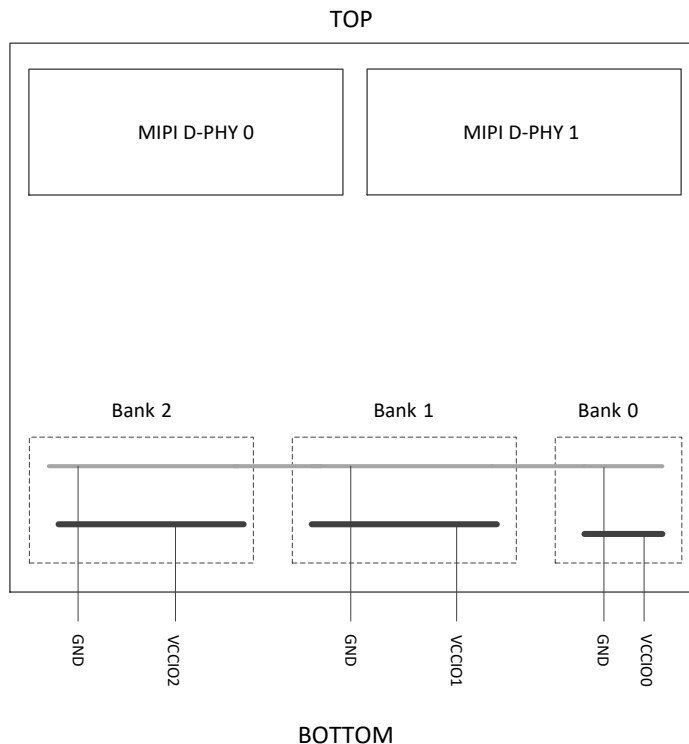
Figure 4.1. sysI/O Banking
